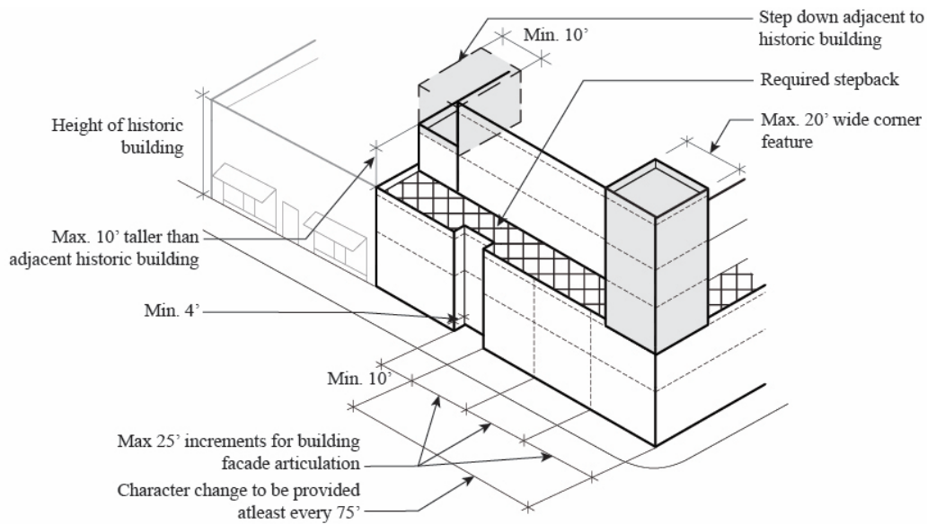
Fig. G.3: Example of steppedown adjacent to historic buildings and taller massing at the block corner.
